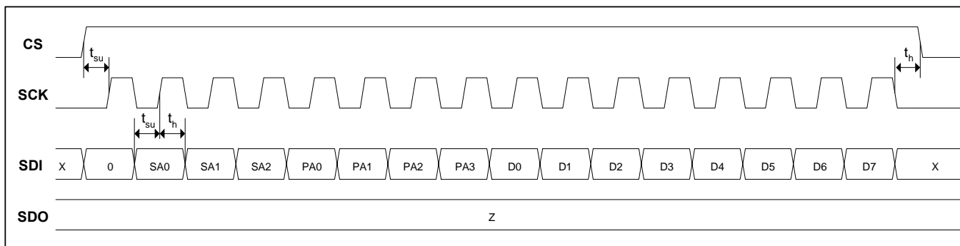
Figure 11: Write Operation
