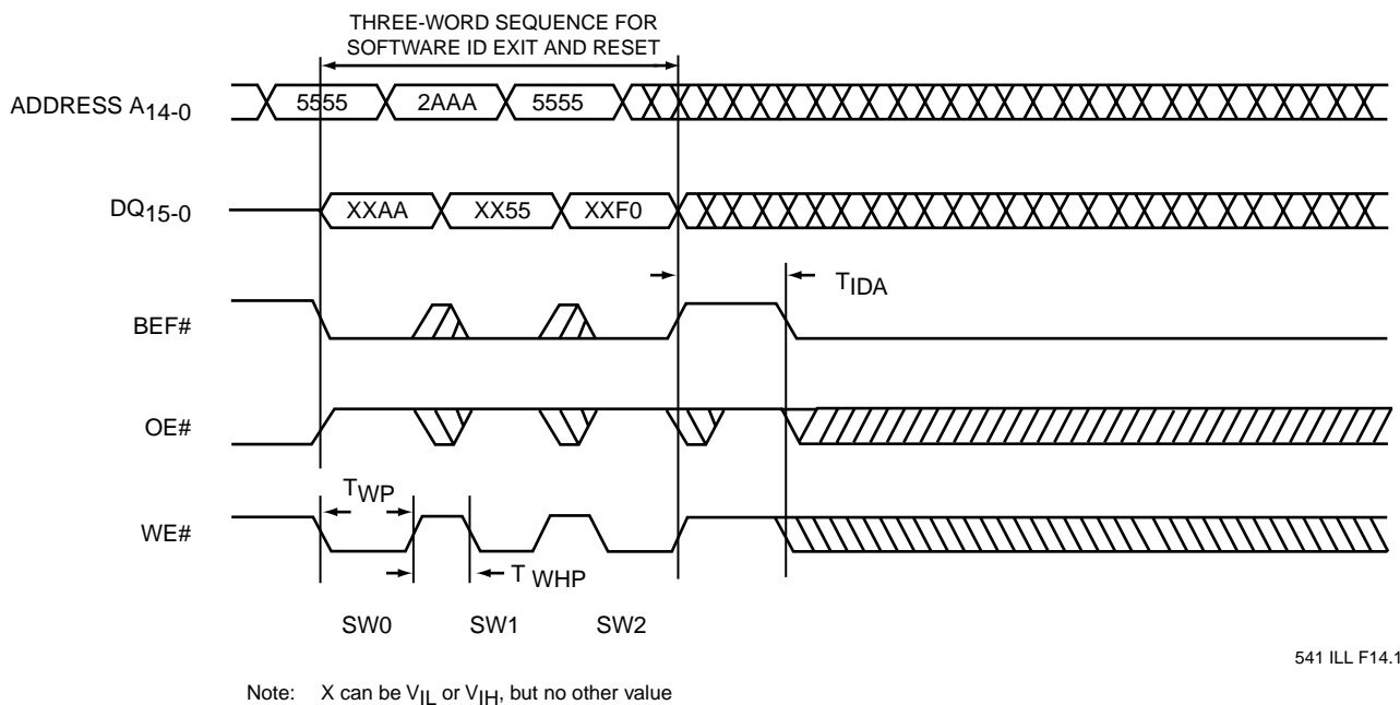
FIGURE 14: SOFTWARE ID EXIT AND RESET
