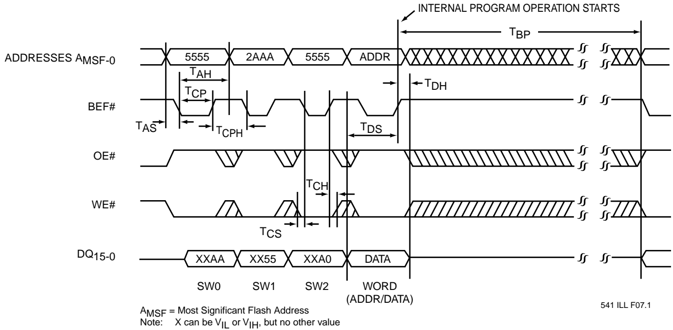
FIGURE 7: BEF# CONTROLLED FLASH PROGRAM CYCLE TIMING DIAGRAM
