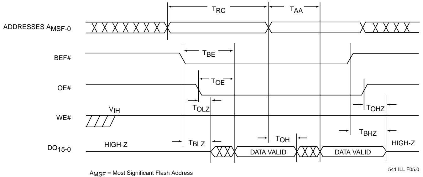
FIGURE 5: FLASH READ CYCLE TIMING DIAGRAM
