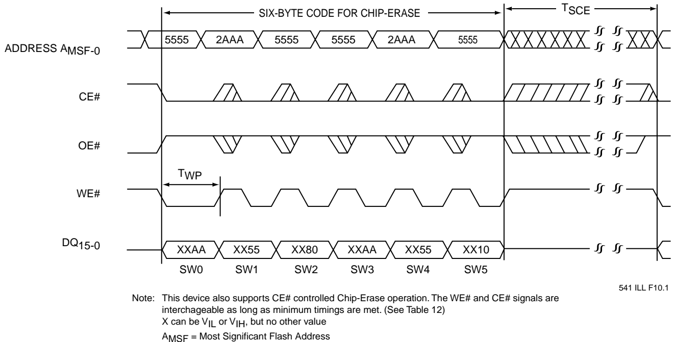
FIGURE 10: WE# CONTROLLED FLASH CHIP-ERASE TIMING DIAGRAM
