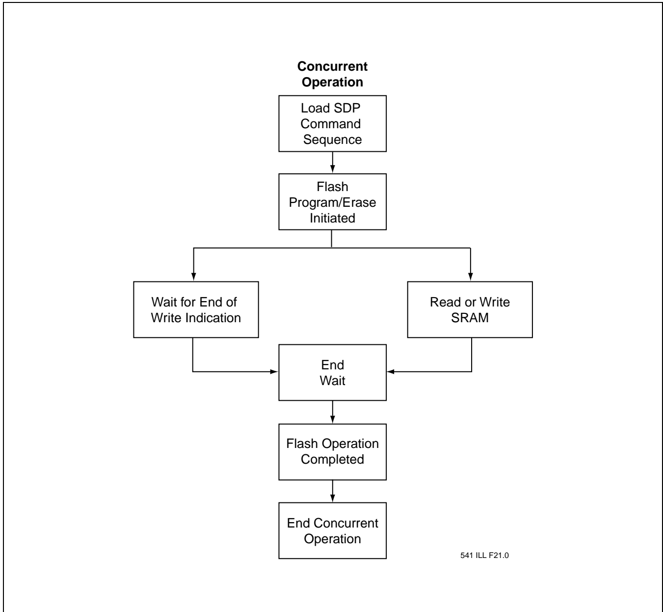
FIGURE 21: CONCURRENT OPERATION FLOWCHART
