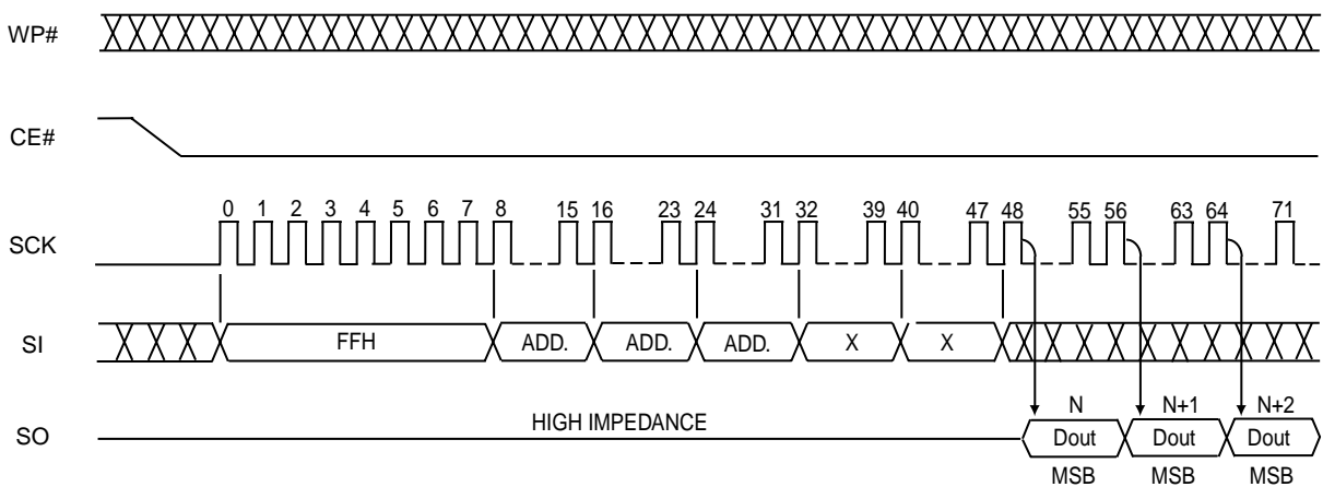
FIGURE 11: READ TIMING DIAGRAM
