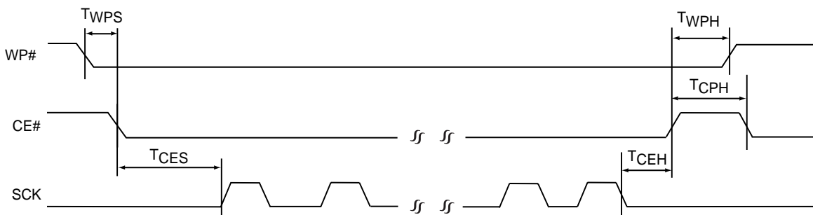
FIGURE 16: WRITE PROTECT TIMING DIAGRAM
