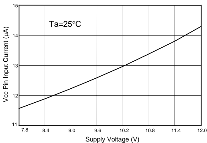
Vcc Pin Input Current vs. Supply Voltage
