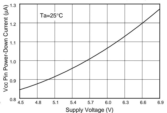
Vcc Pin Power-Down Current vs. Supply Voltage
