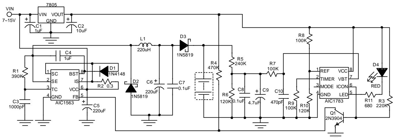
Battery Charge Circuit with Wide Input Voltage Range
