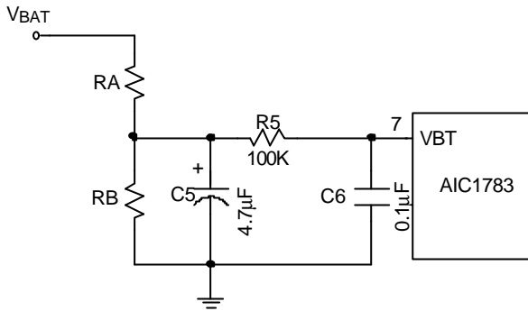
Fig. 1 Battery Voltage Divider
