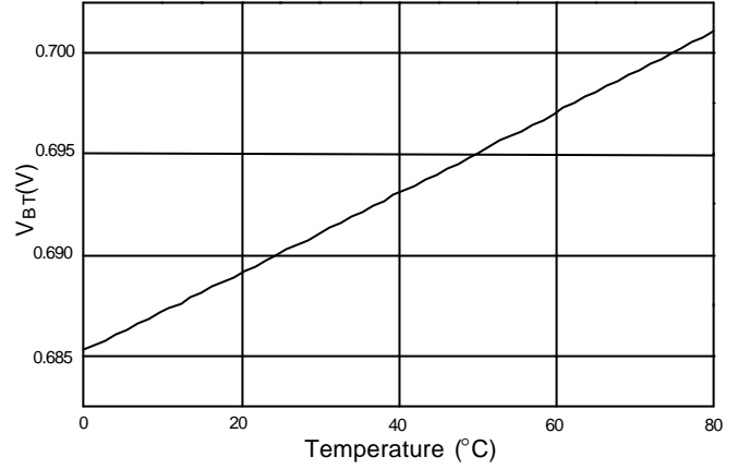
V_{BT(LOW)} Limits vs Temperature (After Initial Timer)
