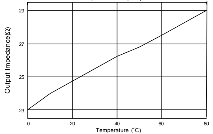
Output Impedance vs Temperature (LED, ICON pins)
