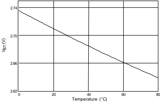
V_{BT} (high) Limit vs Temperature
