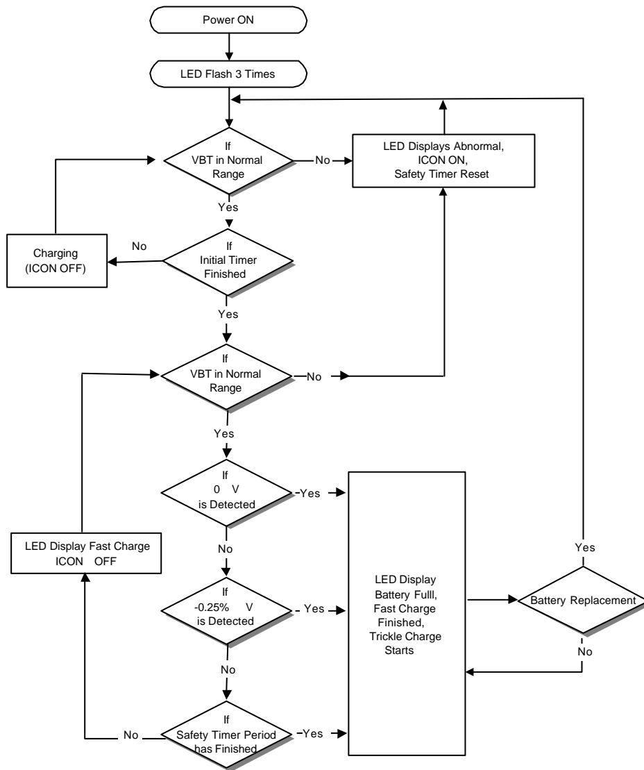
Fig. 2 Function Flow Chart of AIC1783
