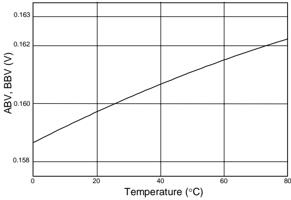
ABV and BBV (Low) Limit vs Temperature (Before Initial Timer)
