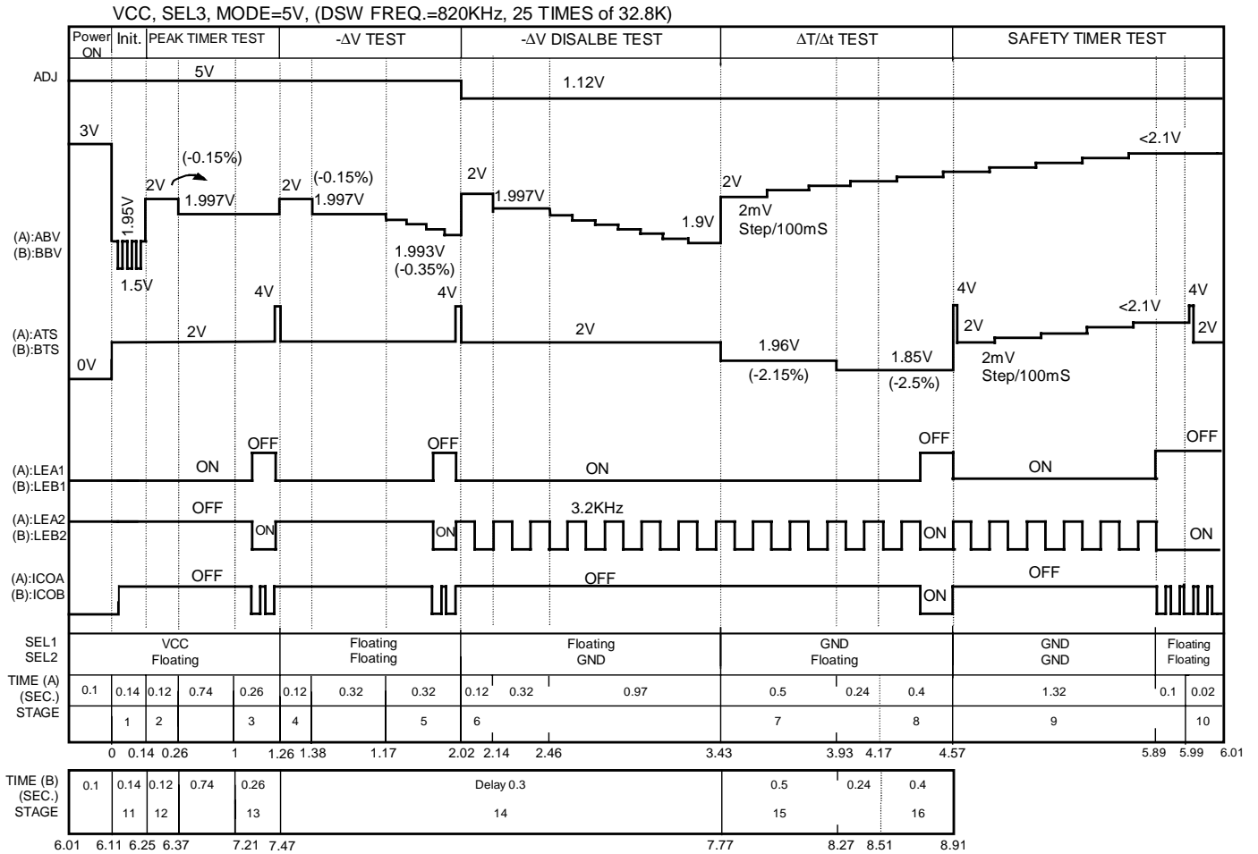
Fig. 5 Timing Diagram of AIC1782 in Test Mode
