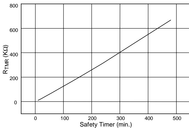
Fig. 4 Safety Timer vs R TMR
