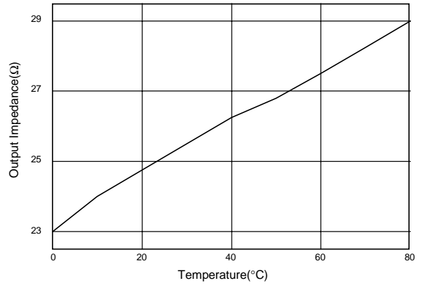
Output Impedance vs Temperature (LEA's, LEB's, ICO's pins)
