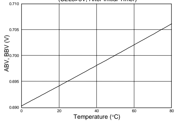
ABV and BBV (Low) limits vs Temperature (SEL3>3V, After Initial Timer)
