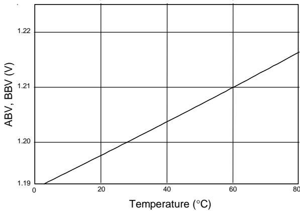
ABV and BBV (Low) limits vs Temperature (SEL3<2V, After Initial Timer)
