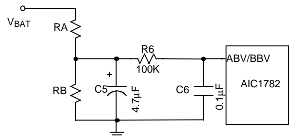
Fig. 2 Battery Voltage Divider
