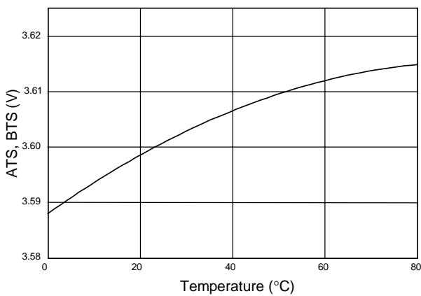
ATS and BTS (High) Limit vs Temperature
