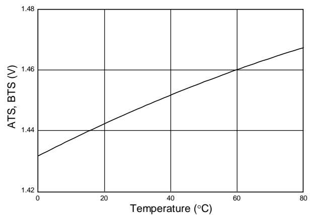
ATS and BTS (Low) Limit vs Temperature
