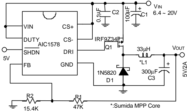
Fig. 1 5V Step-Down Converter
