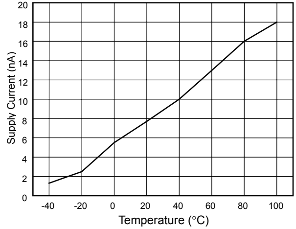
Off-State Supply Current vs. Temperature
