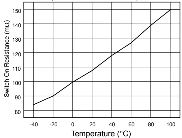
Output On Resistance vs. Temperature
