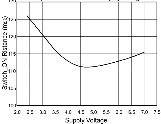
Output On Resistance vs. Supply Voltage
