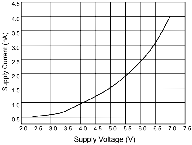
Off-State Supply Current vs. Supply Voltage
