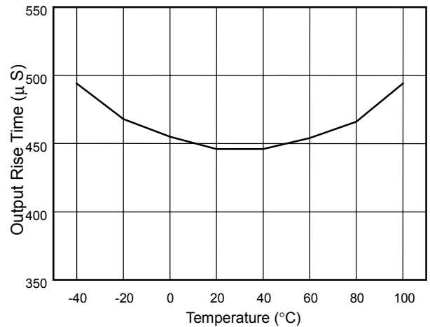
Output Rise Time vs. temperature
